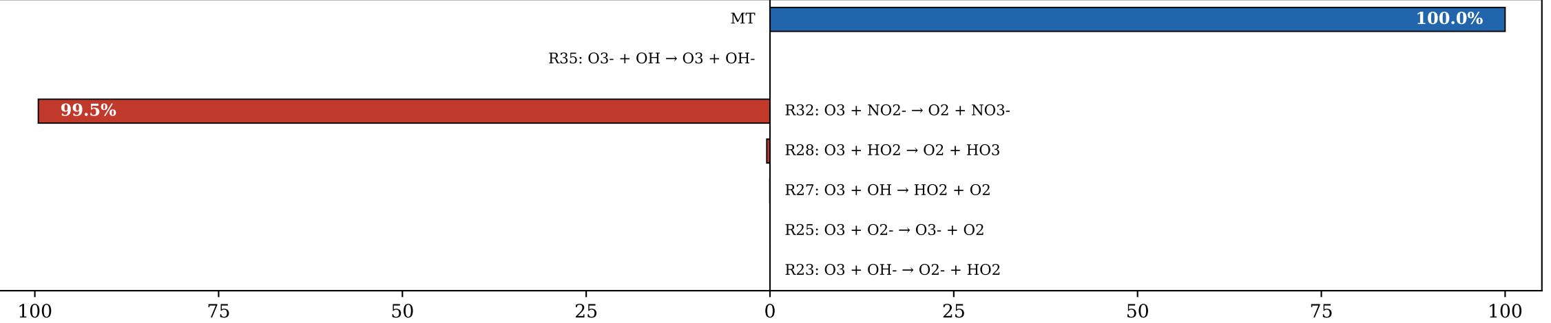
(c) NO 2 - (Σsrc = 3.39e-07 M/s)
